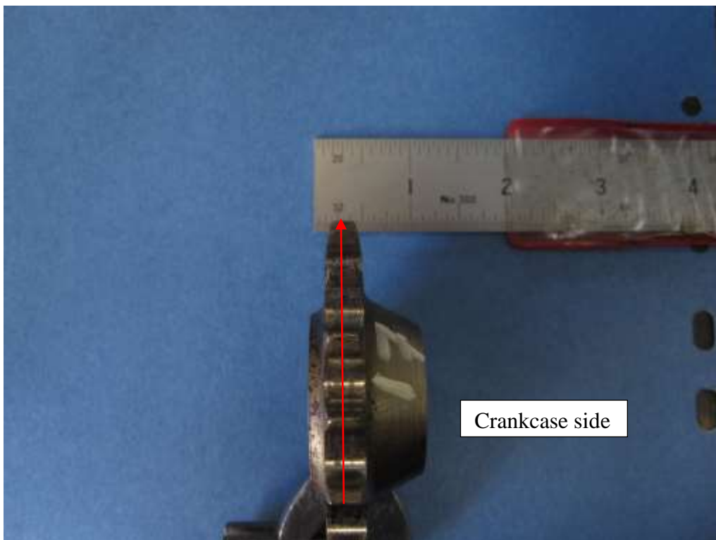
Figure two. Engine sprocket, top view, 17 teeth; center line of chain path appears to be ~ 1" in from the crank case side and ~1/4" from primary case / alternator rotor.
