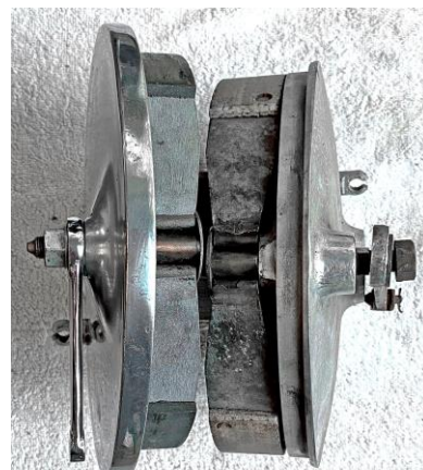
Alloy Brake Plates – Full Width Hubs LHS: 1954-55, RHS: 1956-70
